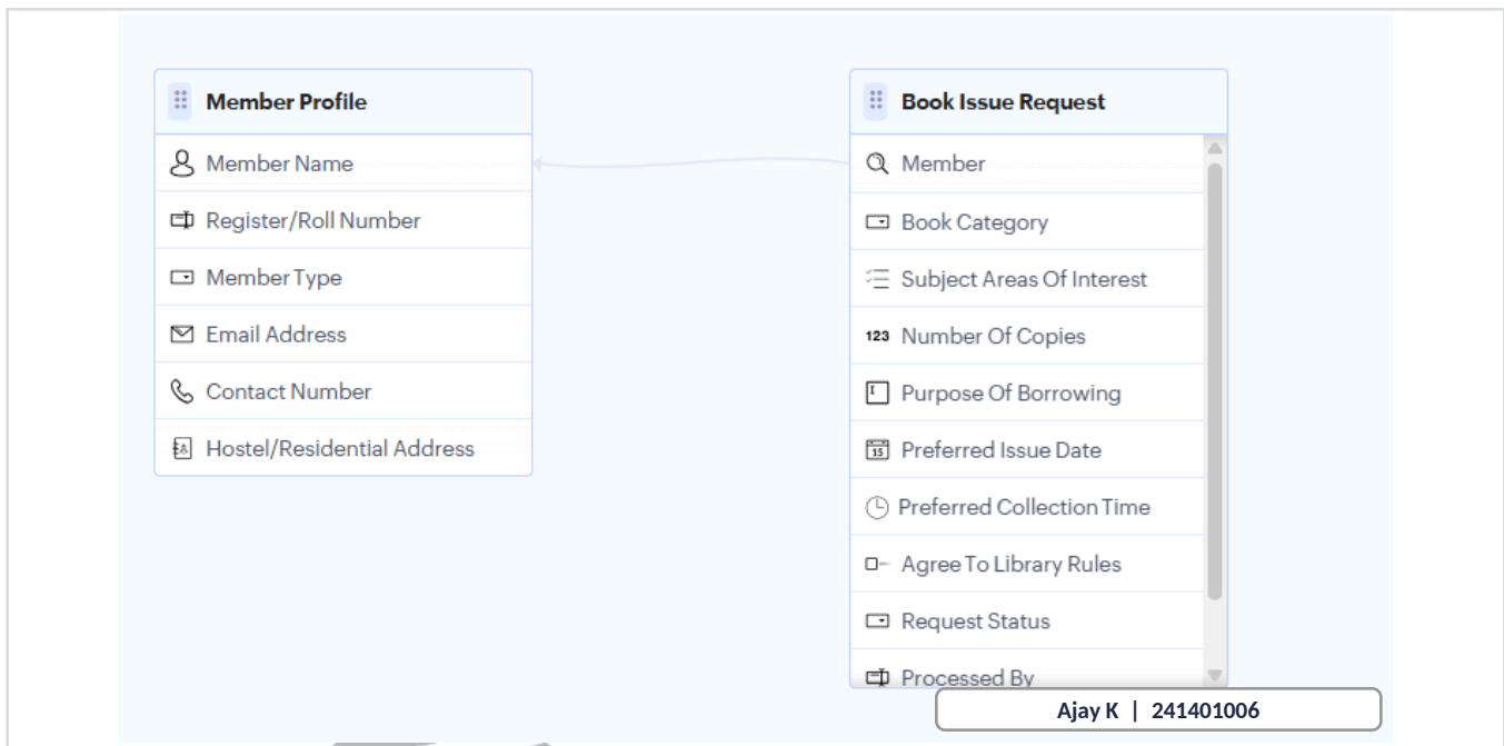
Fig. 1 — Data model showing the Member Profile and Book Issue Request forms and their lookup relationship
